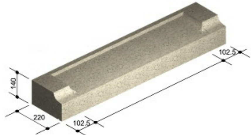
Brick Ope Isometric view of Timber-Frame Stooled Sill
