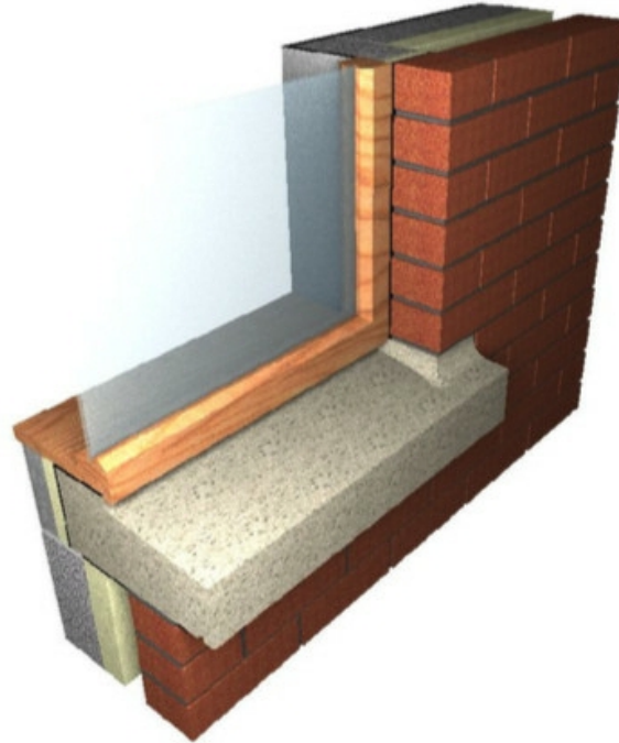
Section Detail by In Granite Recon Cavity Wall Construction - Brick Outer Leaf using 140mm Stooled Sill
